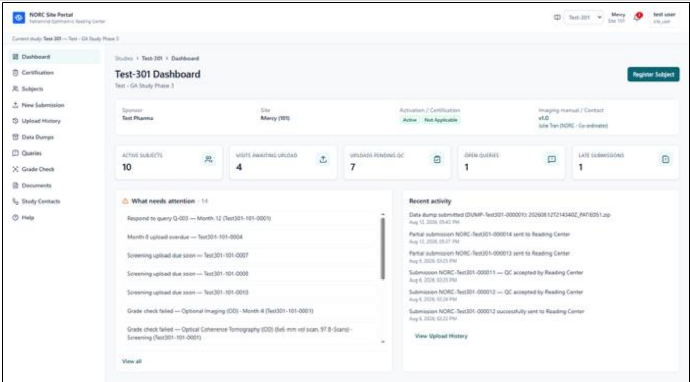
Figure 7. Study dashboard
