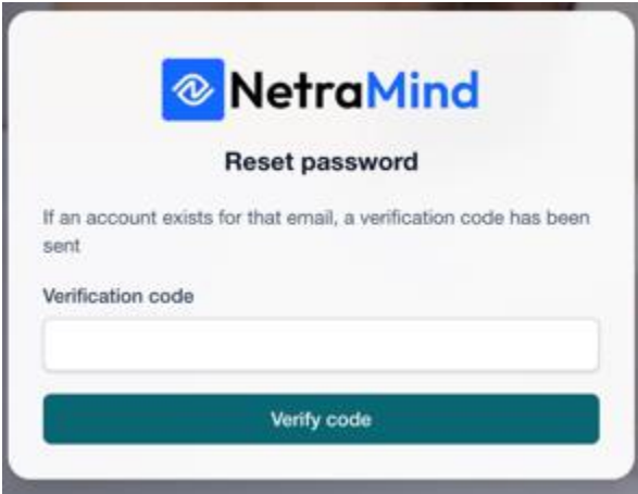
Figure 5. Reset password
