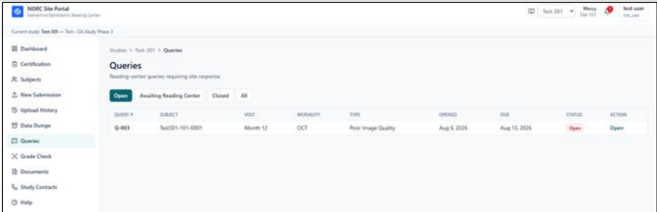
Figure 29. Queries dashboard
